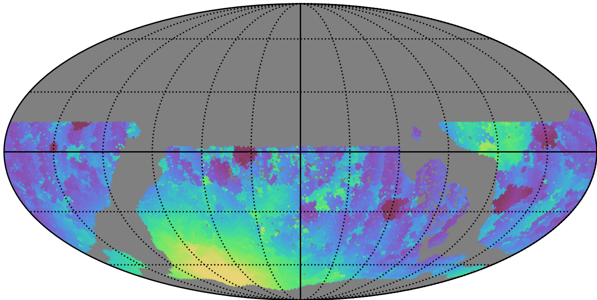
too_elab_r32_d2_giz_v3.4_10yrs WFD g band: Min moonDistance
