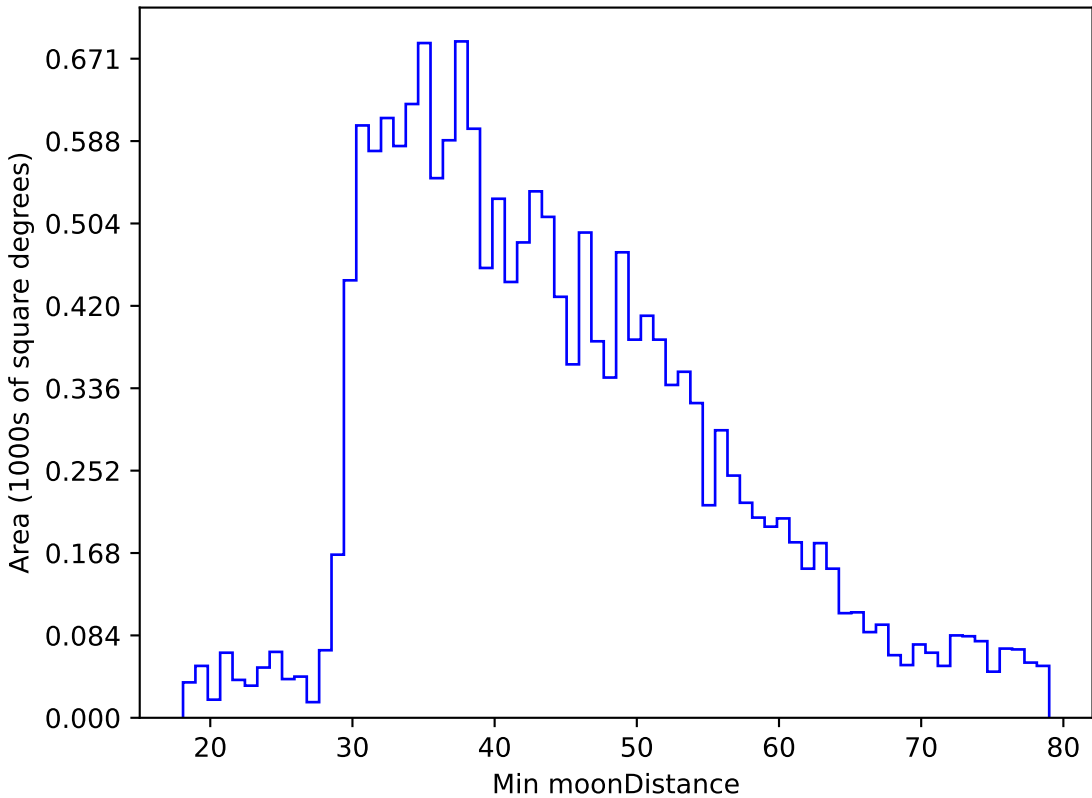
too_elab_r32_d2_giz_v3.4_10yrs WFD g band: Min moonDistance
