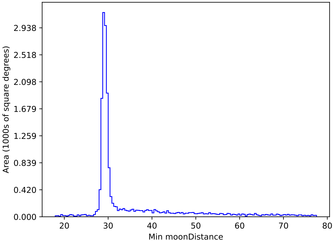
too_elab_r32_d2_giz_v3.4_10yrs WFD all bands: Min moonDistance
