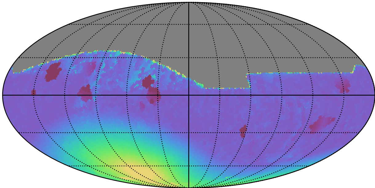
too_elab_r32_d2_giz_v3.4_10yrs All sky z band: Min moonDistance
