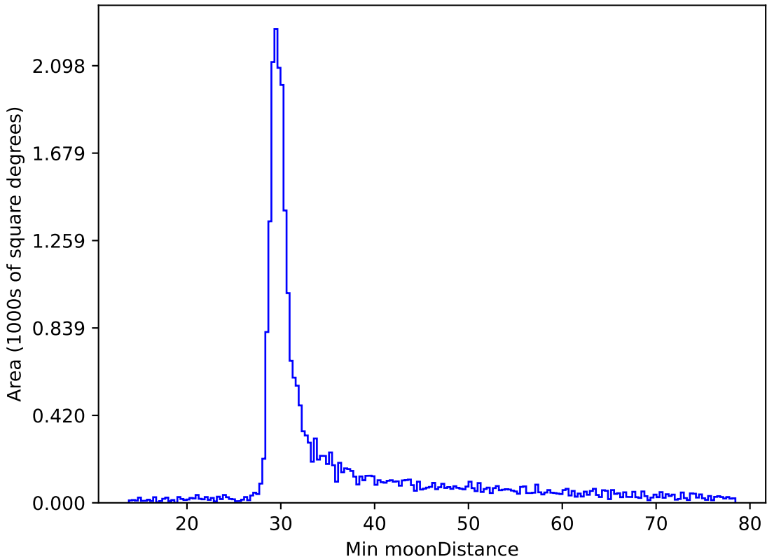
too_elab_r32_d2_giz_v3.4_10yrs All sky z band: Min moonDistance
