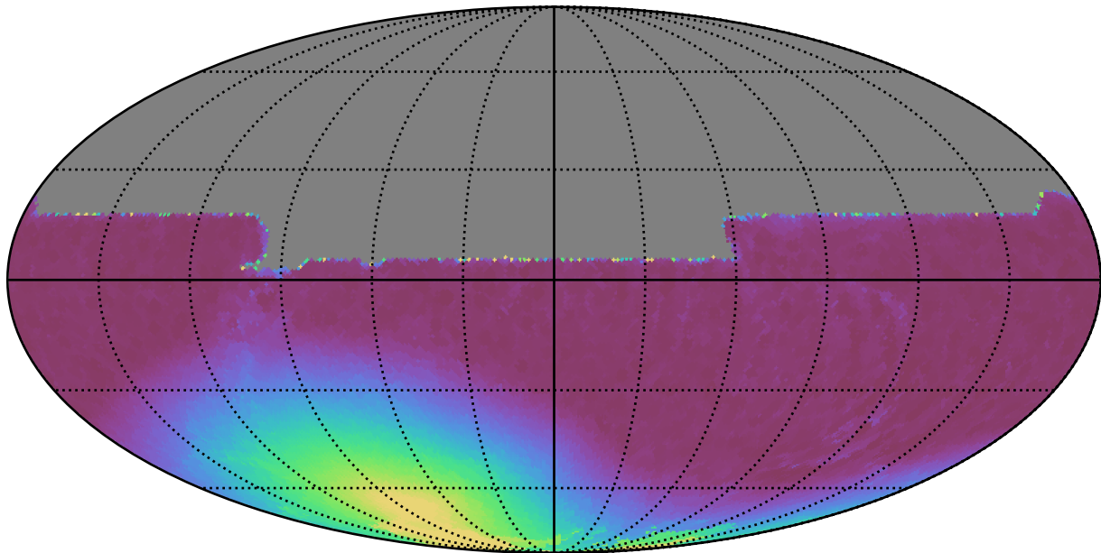
too_elab_r32_d2_giz_v3.4_10yrs All sky y band: Min moonDistance
