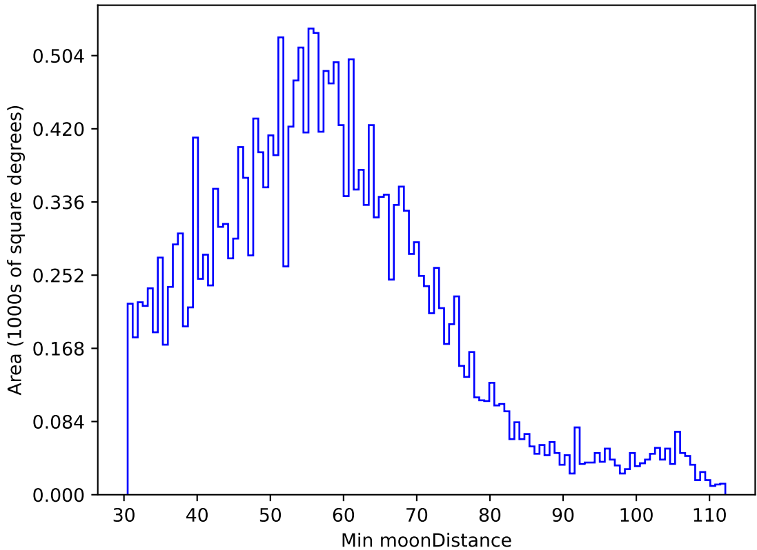
too_elab_r32_d2_giz_v3.4_10yrs All sky u band: Min moonDistance
