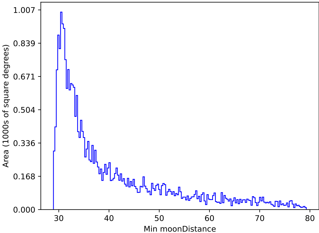
too_elab_r32_d2_giz_v3.4_10yrs All sky r band: Min moonDistance
