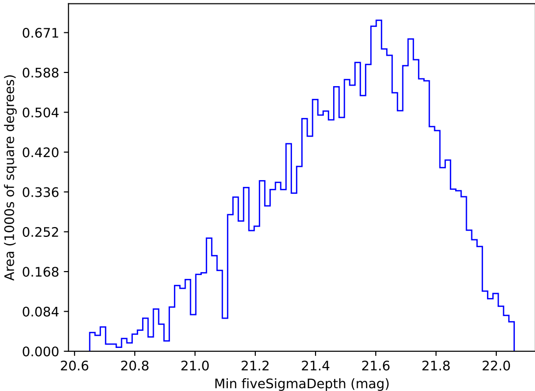
too_elab_r32_d2_giz_v3.4_10yrs Yr 1 y band: Min fiveSigmaDepth
