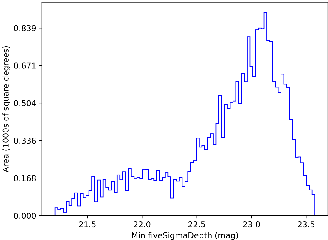
too_elab_r32_d2_giz_v3.4_10yrs Yr 1 i band: Min fiveSigmaDepth
