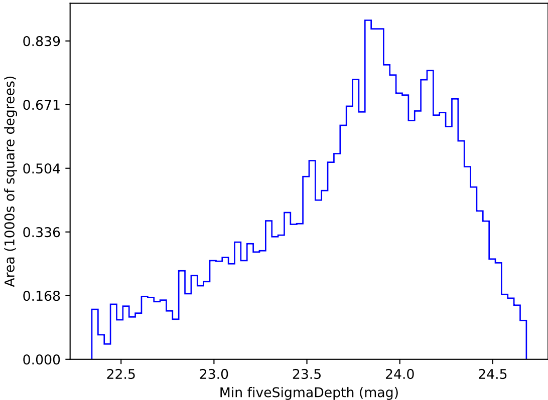
too_elab_r32_d2_giz_v3.4_10yrs Yr 1 g band: Min fiveSigmaDepth
