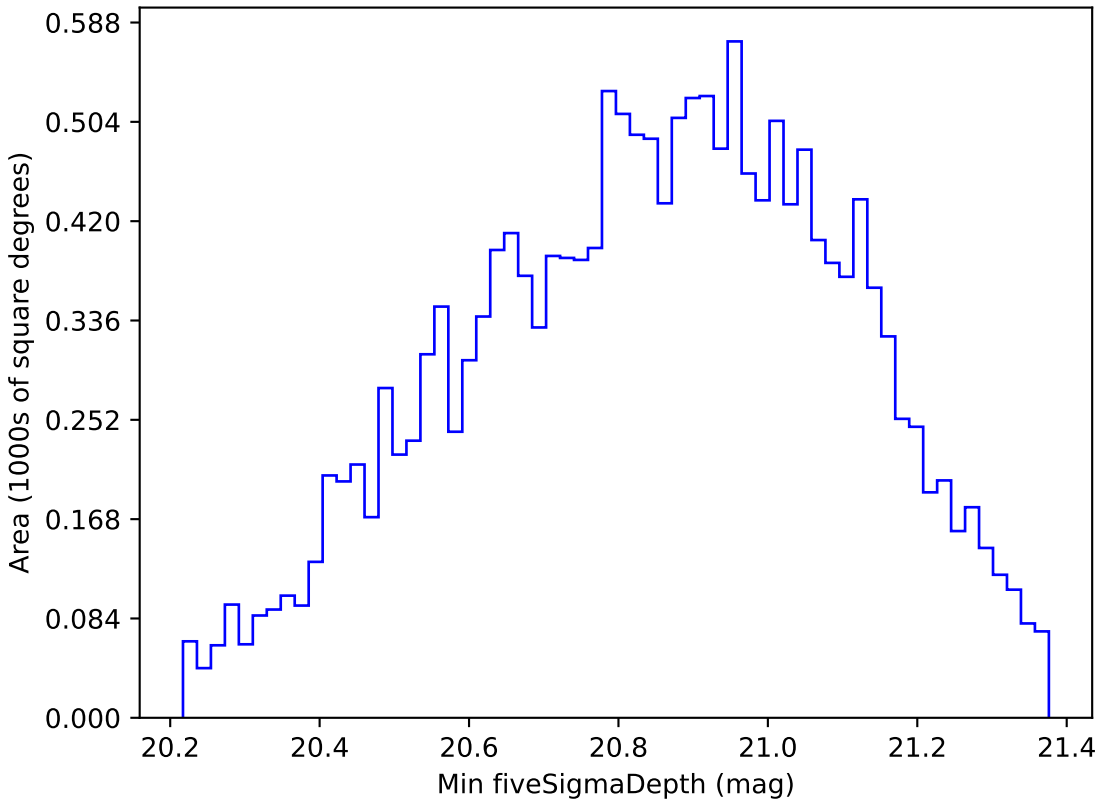
too_elab_r32_d2_giz_v3.4_10yrs WFD y band: Min fiveSigmaDepth
