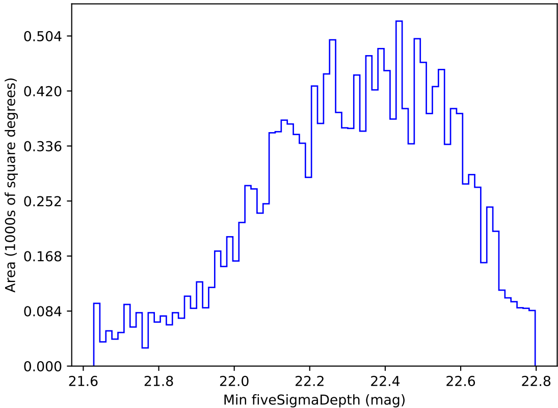
too_elab_r32_d2_giz_v3.4_10yrs WFD u band: Min fiveSigmaDepth
