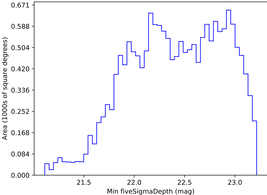
too_elab_r32_d2_giz_v3.4_10yrs WFD r band: Min fiveSigmaDepth
