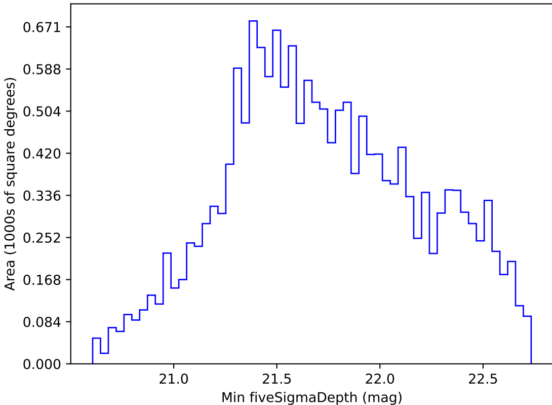
too_elab_r32_d2_giz_v3.4_10yrs WFD i band: Min fiveSigmaDepth
