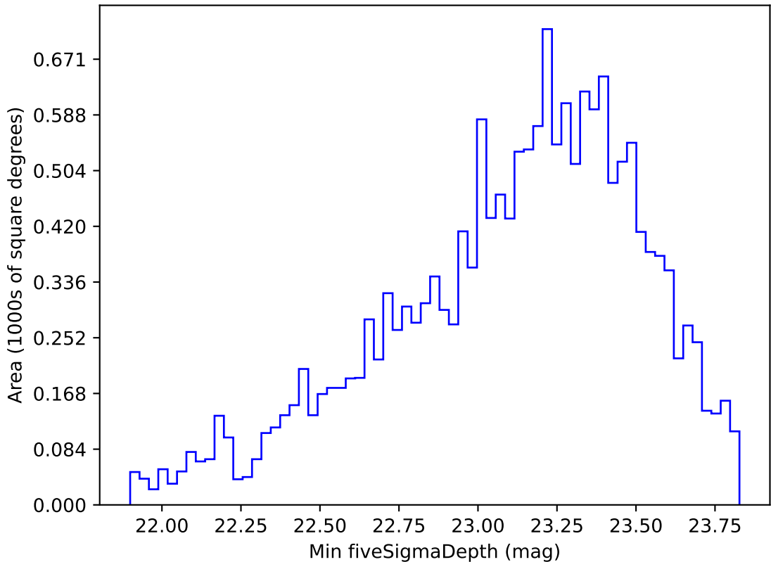
too_elab_r32_d2_giz_v3.4_10yrs WFD g band: Min fiveSigmaDepth
