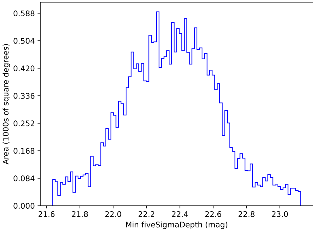
too_elab_r32_d2_giz_v3.4_10yrs All sky u band: Min fiveSigmaDepth
