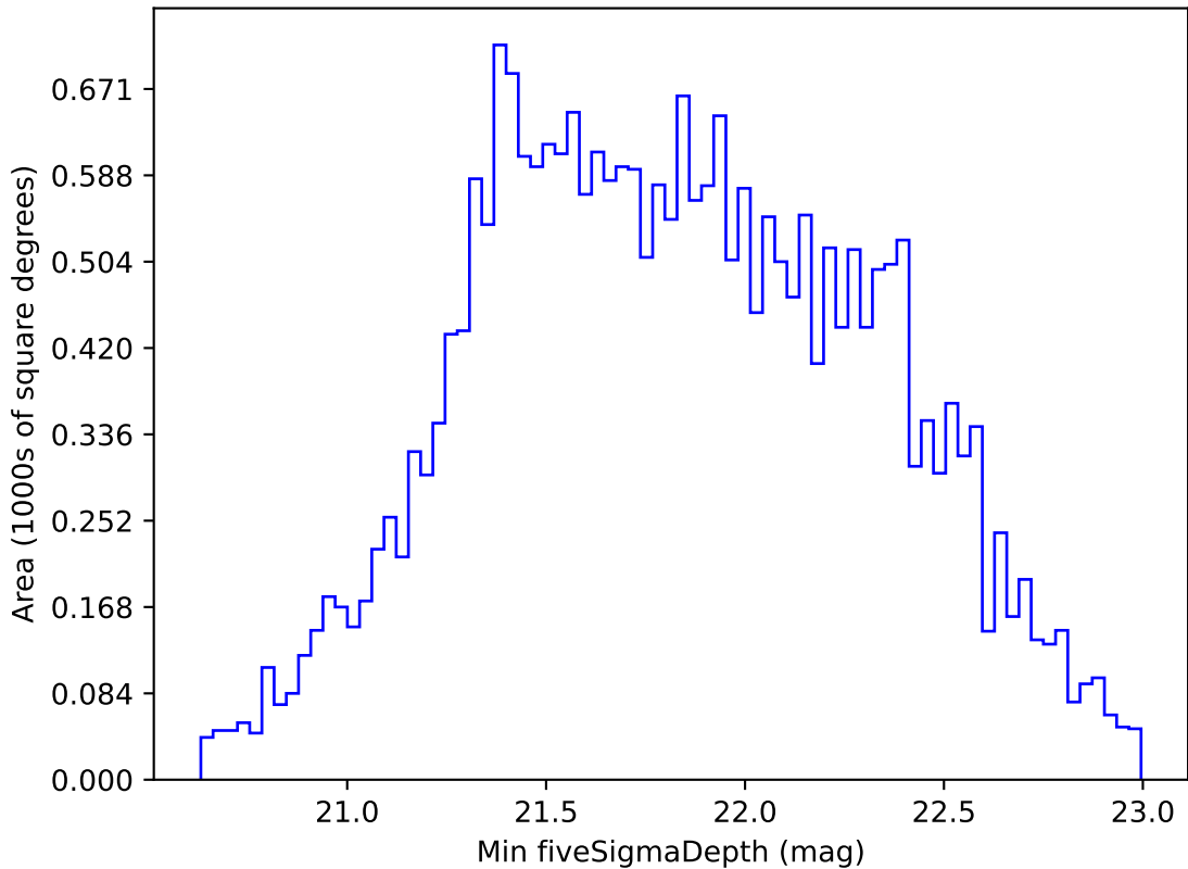
too_elab_r32_d2_giz_v3.4_10yrs All sky i band: Min fiveSigmaDepth
