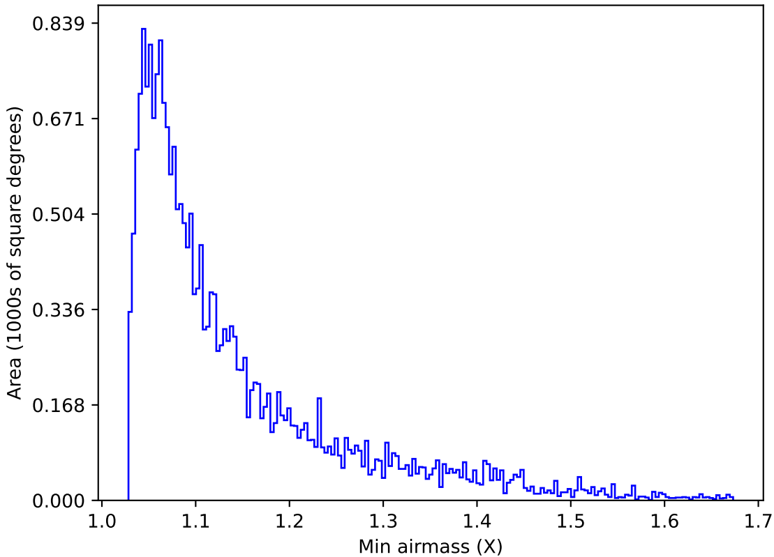
too_elab_r32_d2_giz_v3.4_10yrs Yr 1 u band: Min airmass
