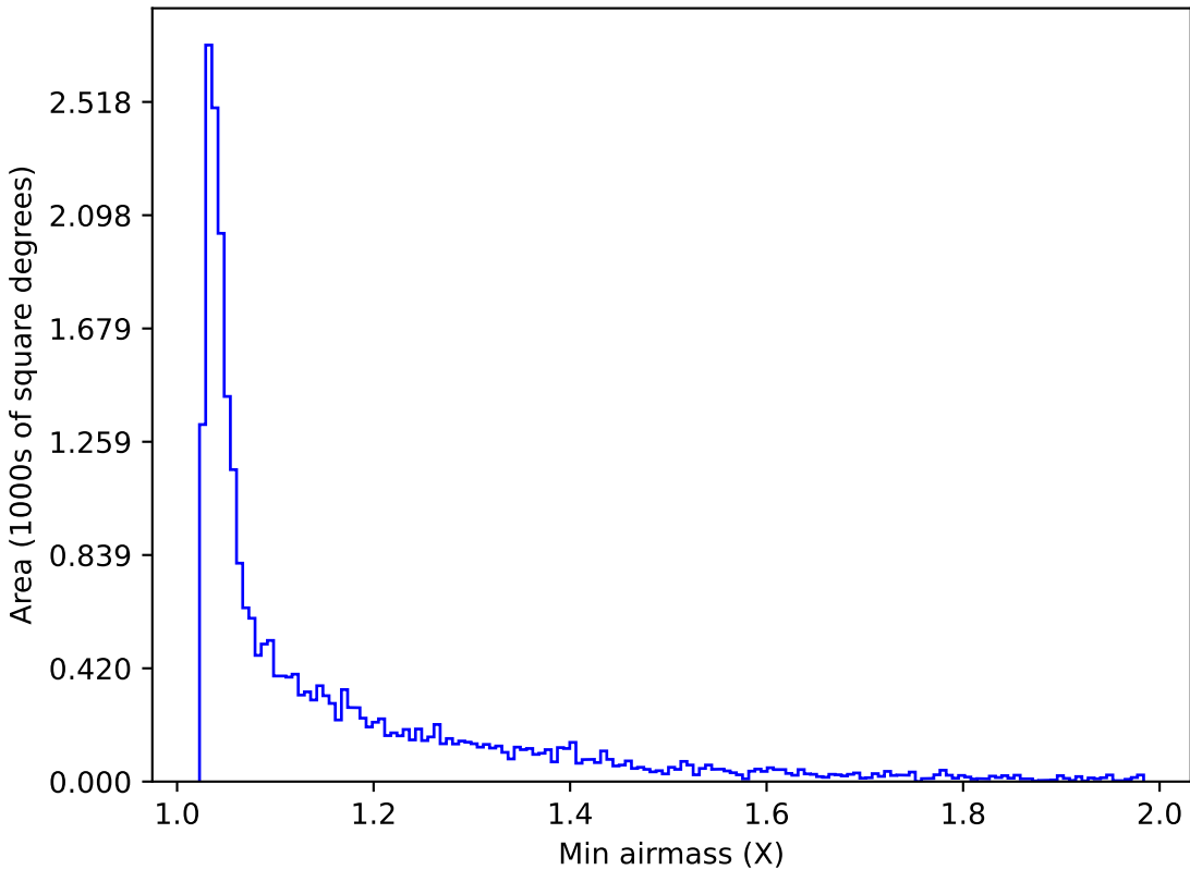
too_elab_r32_d2_giz_v3.4_10yrs Yr 1 r band: Min airmass
