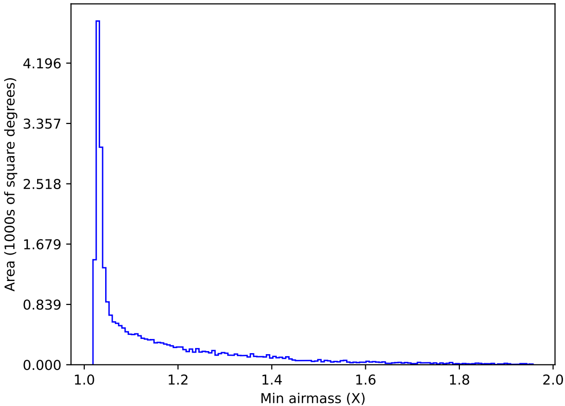
too_elab_r32_d2_giz_v3.4_10yrs Yr 1 all bands: Min airmass
