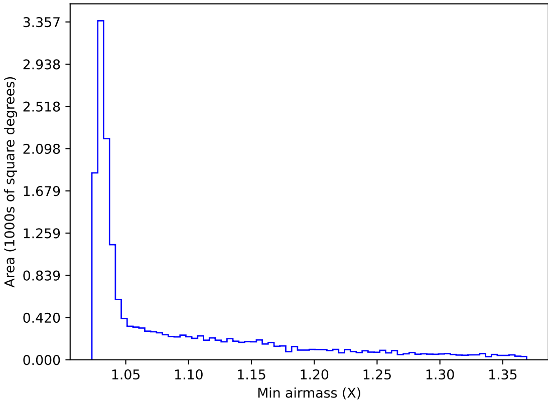
too_elab_r32_d2_giz_v3.4_10yrs WFD y band: Min airmass
