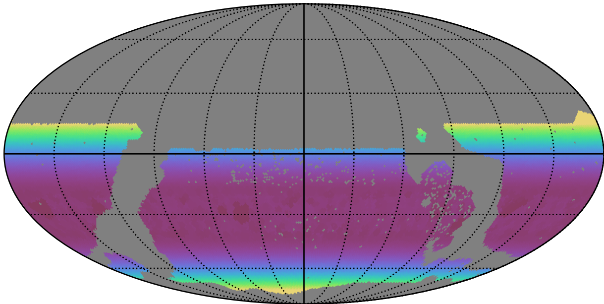
too_elab_r32_d2_giz_v3.4_10yrs WFD all bands: Min airmass
