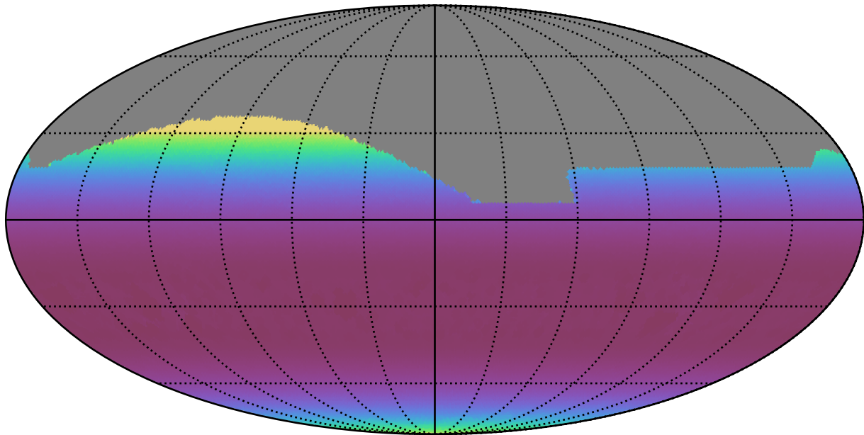
too_elab_r32_d2_giz_v3.4_10yrs All sky all bands: Min airmass
