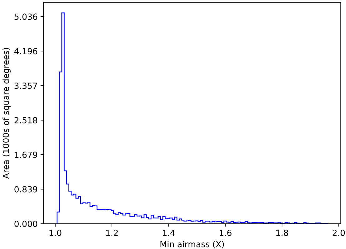
too_elab_r32_d2_giz_v3.4_10yrs All sky all bands: Min airmass
