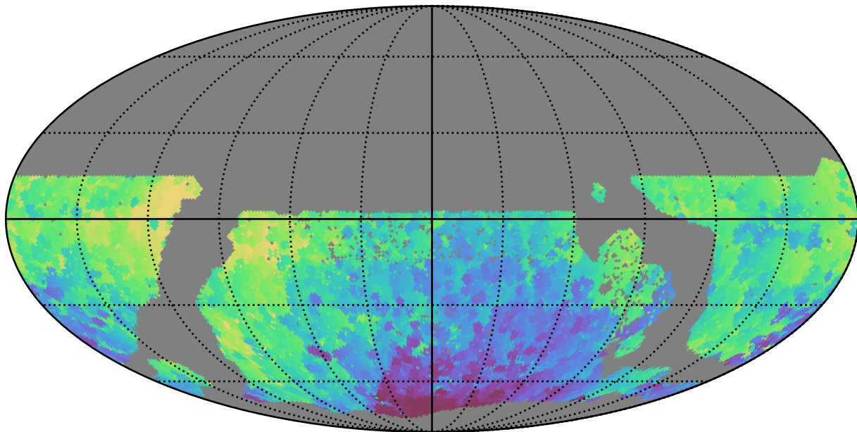
too_elab_r32_d2_giz_v3.4_10yrs WFD y band: Min HA
