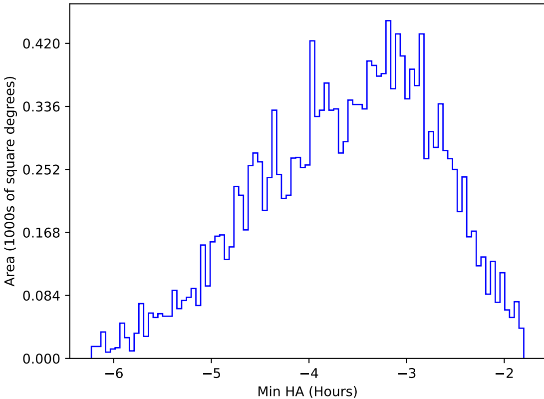
too_elab_r32_d2_giz_v3.4_10yrs WFD y band: Min HA
