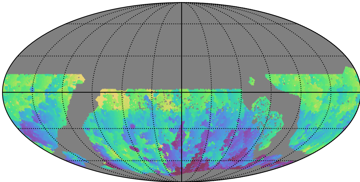
too_elab_r32_d2_giz_v3.4_10yrs WFD u band: Min HA
