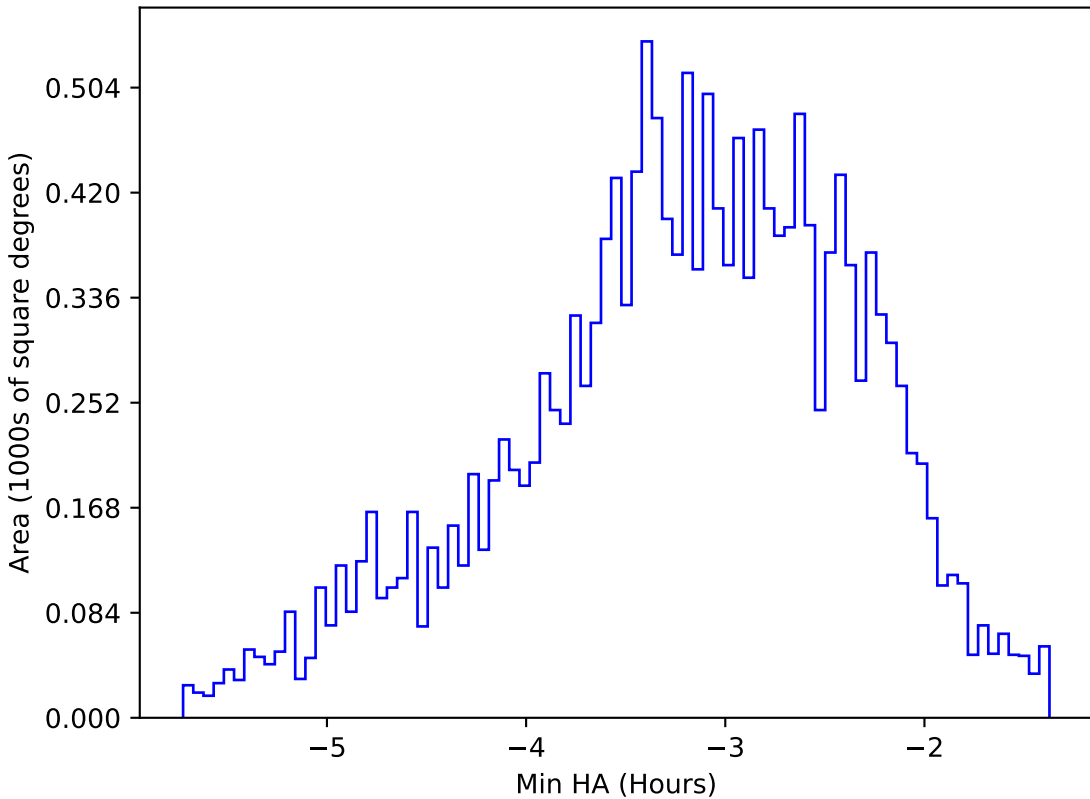
too_elab_r32_d2_giz_v3.4_10yrs WFD u band: Min HA
