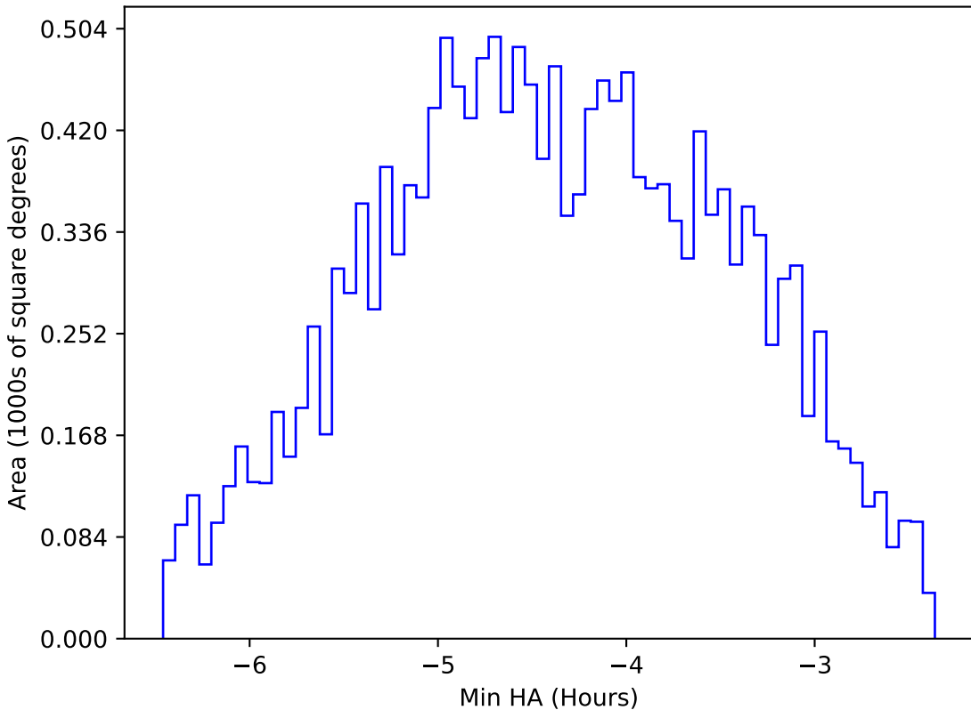
too_elab_r32_d2_giz_v3.4_10yrs WFD i band: Min HA
