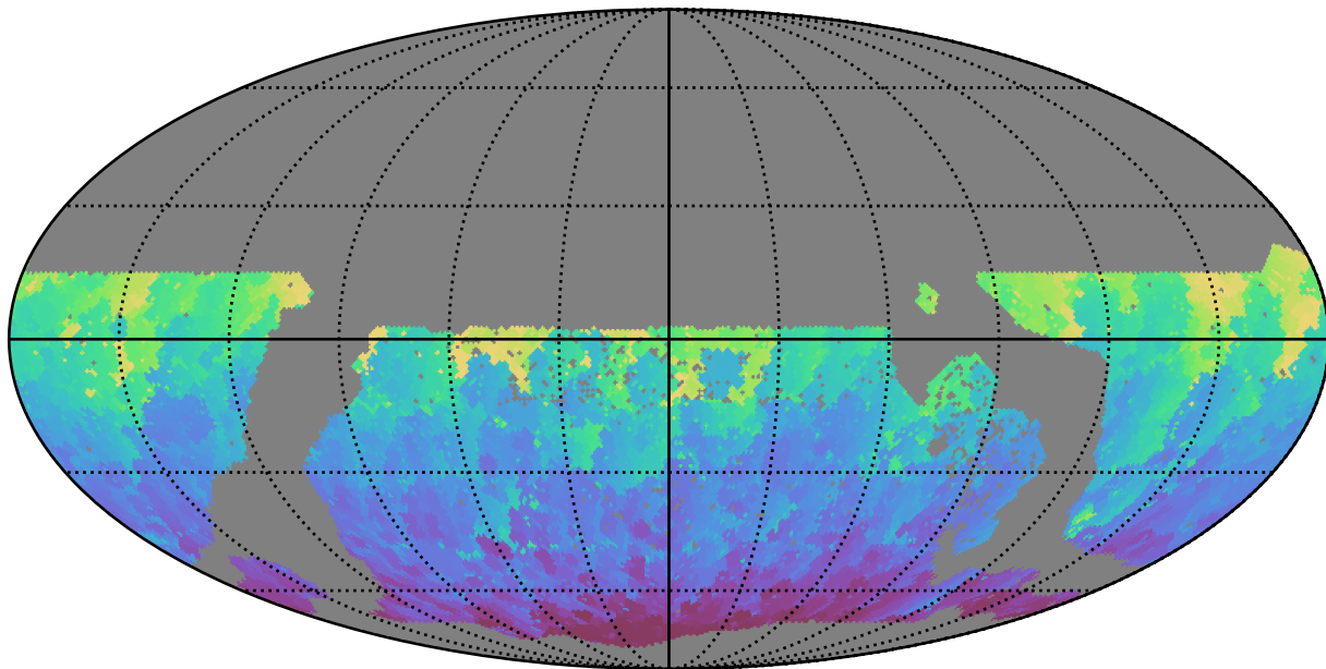
too_elab_r32_d2_giz_v3.4_10yrs WFD g band: Min HA
