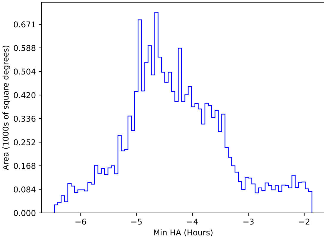
too_elab_r32_d2_giz_v3.4_10yrs WFD g band: Min HA
