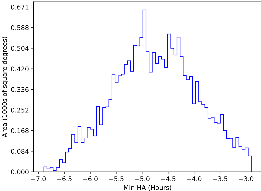
too_elab_r32_d2_giz_v3.4_10yrs WFD all bands: Min HA
