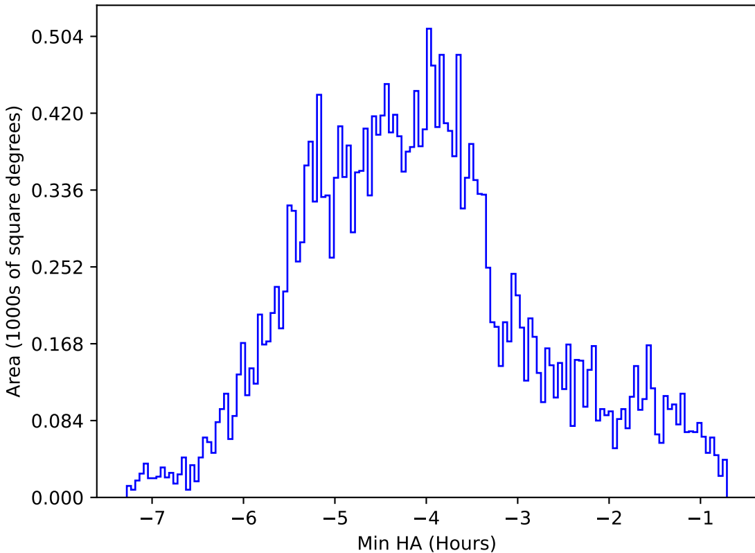
too_elab_r32_d2_giz_v3.4_10yrs All sky z band: Min HA
