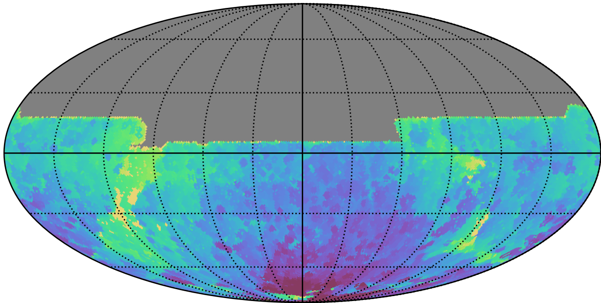
too_elab_r32_d2_giz_v3.4_10yrs All sky y band: Min HA
