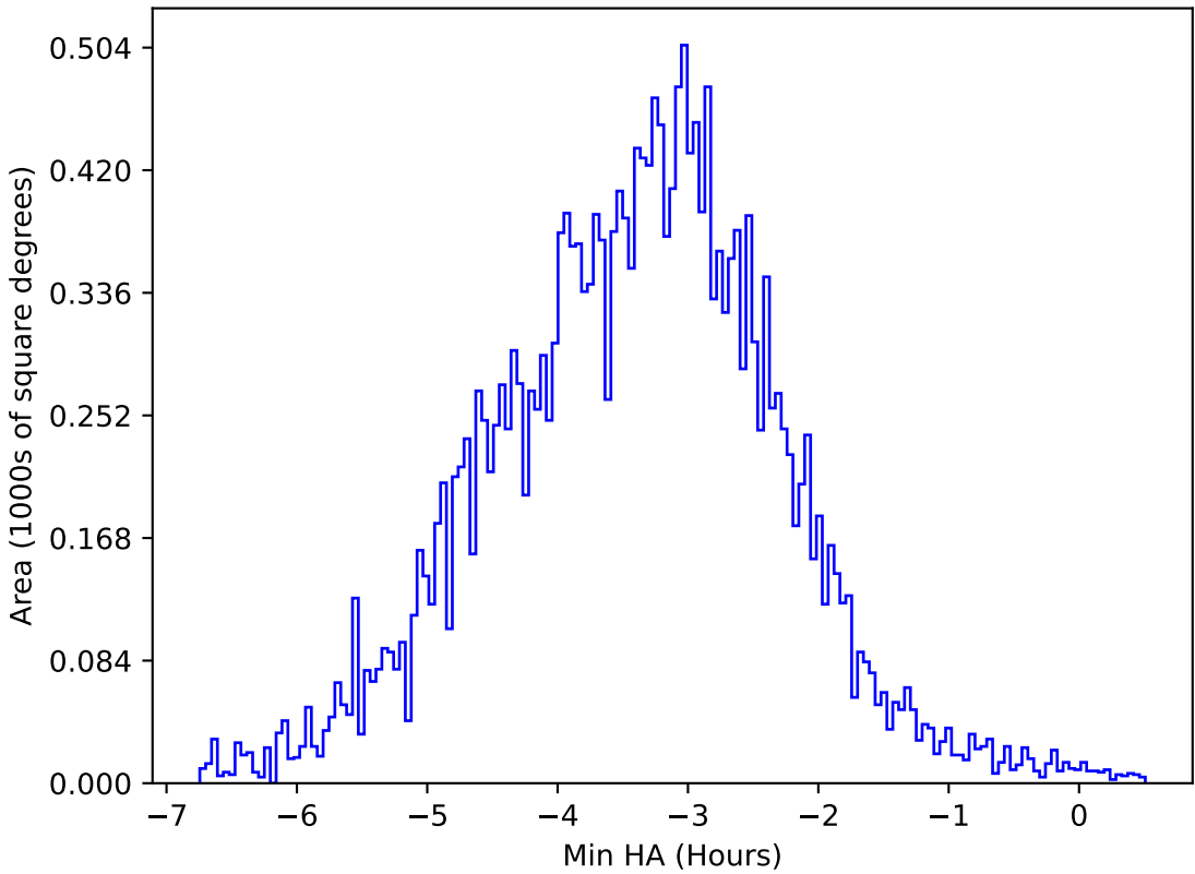
too_elab_r32_d2_giz_v3.4_10yrs All sky y band: Min HA
