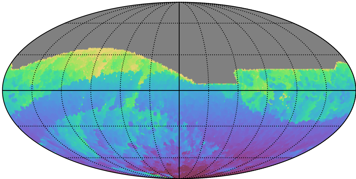
too_elab_r32_d2_giz_v3.4_10yrs All sky r band: Min HA
