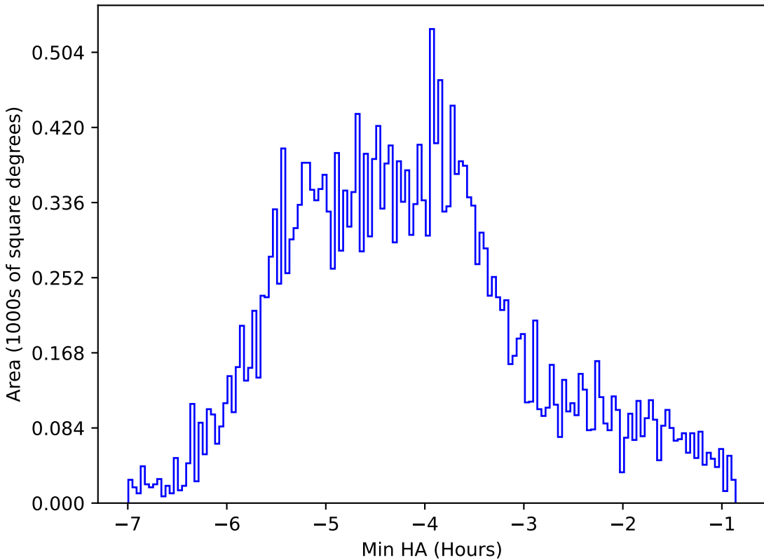
too_elab_r32_d2_giz_v3.4_10yrs All sky r band: Min HA
