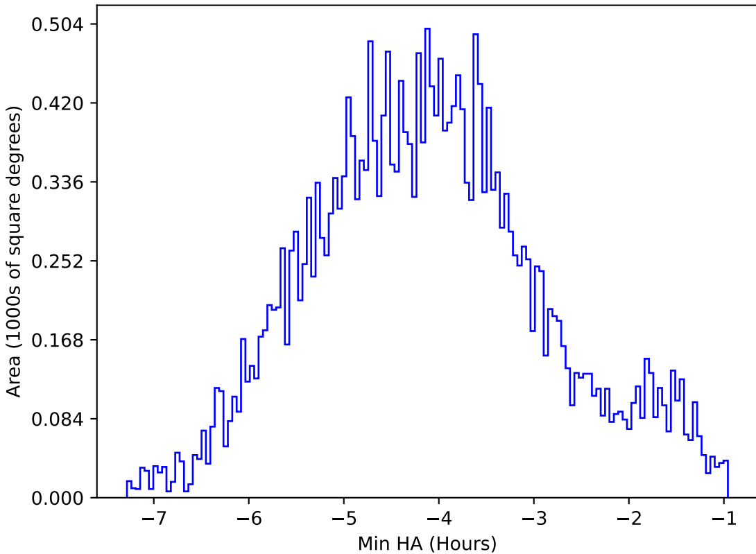
too_elab_r32_d2_giz_v3.4_10yrs All sky i band: Min HA
