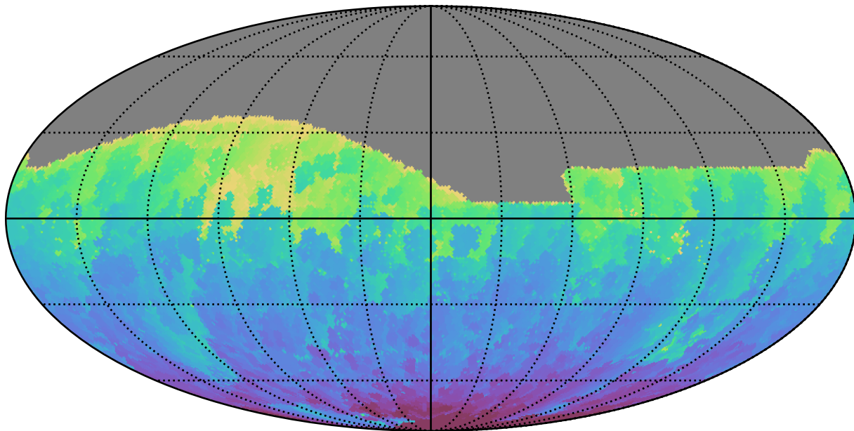
too_elab_r32_d2_giz_v3.4_10yrs All sky g band: Min HA
