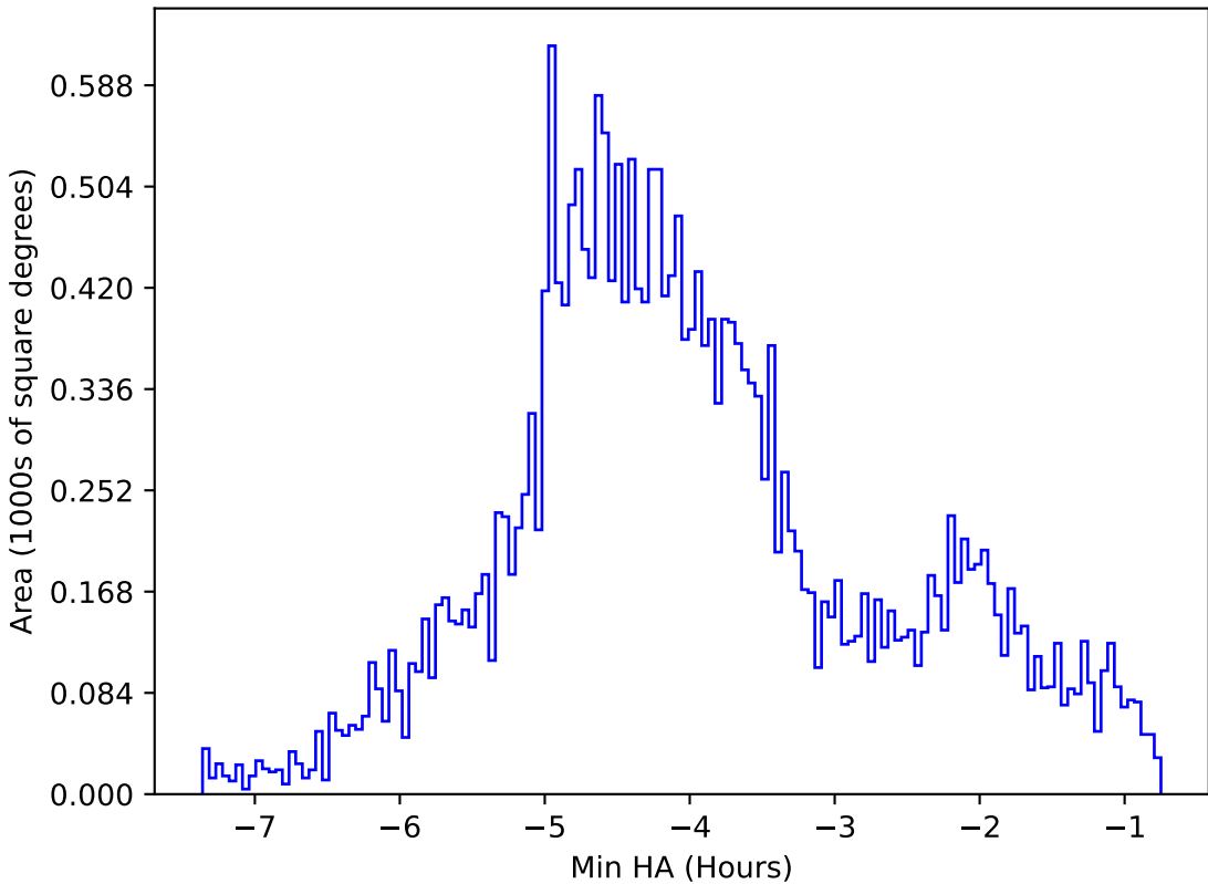
too_elab_r32_d2_giz_v3.4_10yrs All sky g band: Min HA
