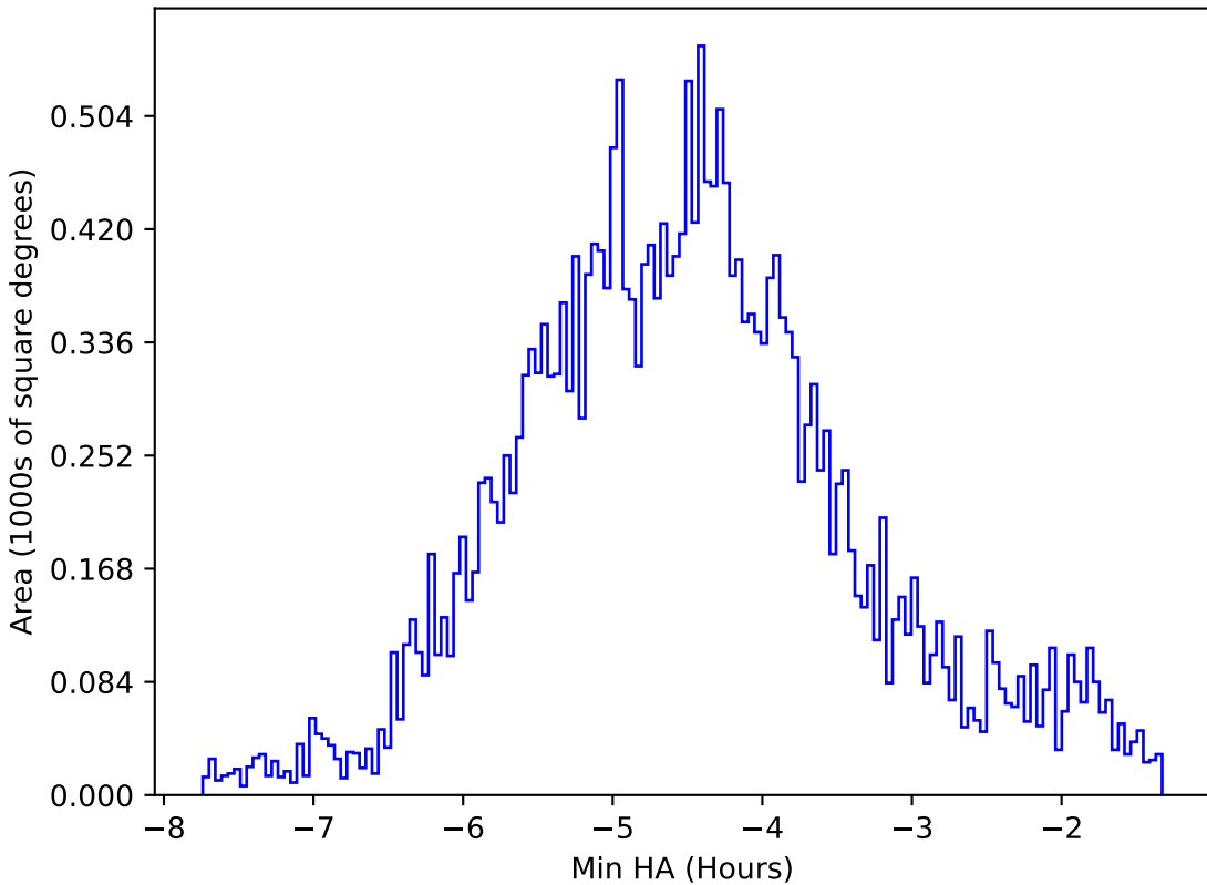
too_elab_r32_d2_giz_v3.4_10yrs All sky all bands: Min HA
