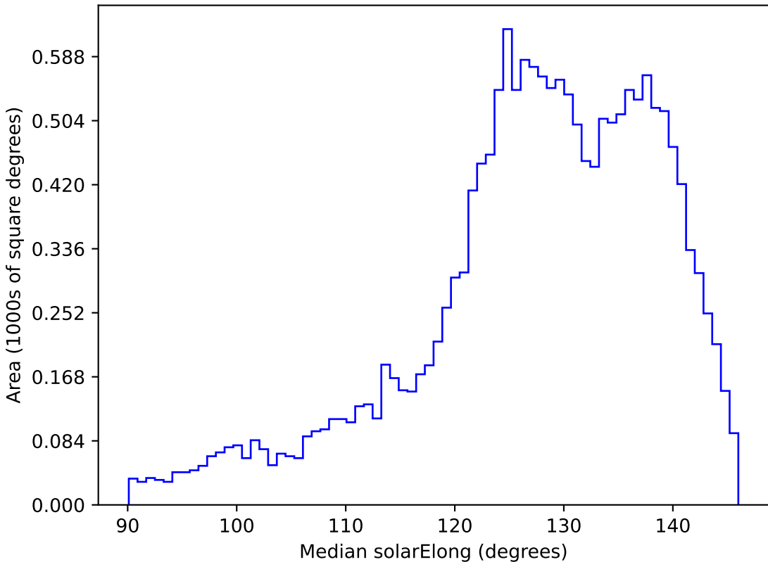
too_elab_r32_d2_giz_v3.4_10yrs WFD z band: Median solarElong
