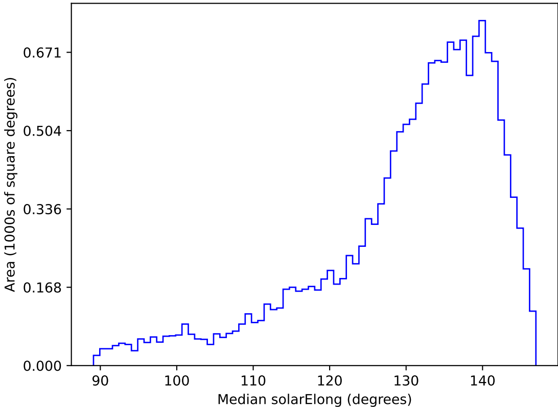
too_elab_r32_d2_giz_v3.4_10yrs WFD y band: Median solarElong
