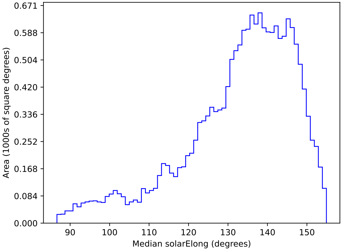
too_elab_r32_d2_giz_v3.4_10yrs WFD u band: Median solarElong
