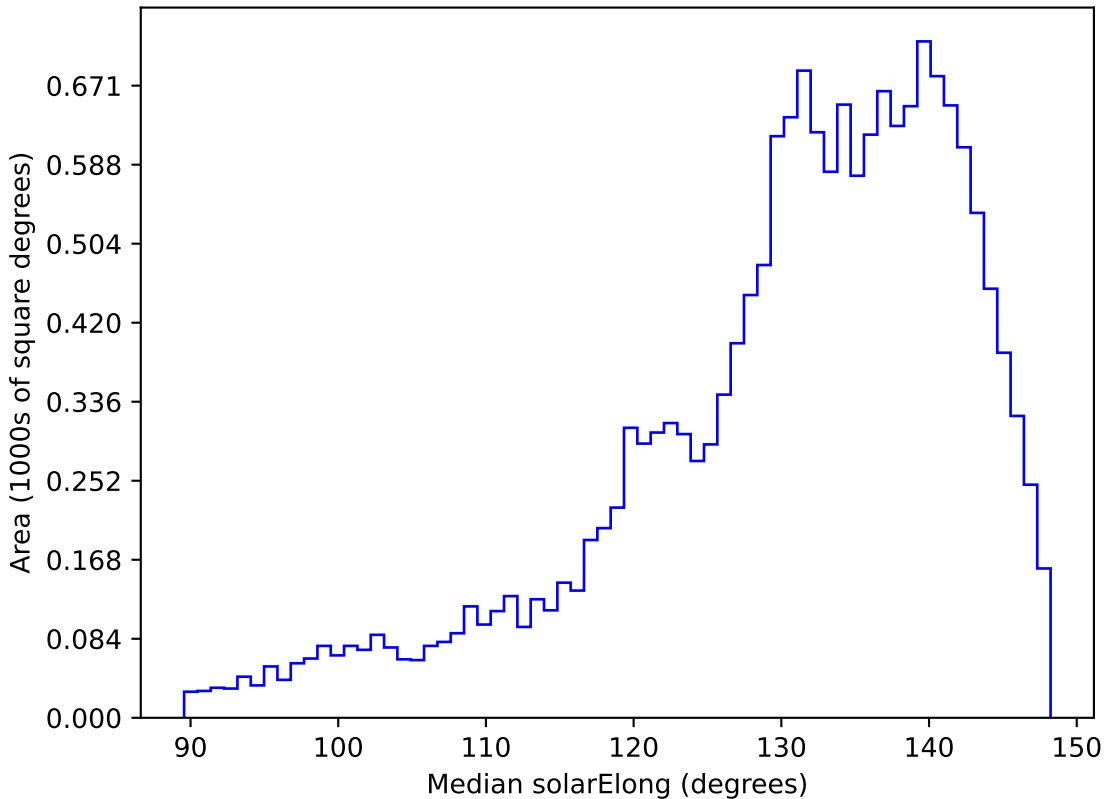
too_elab_r32_d2_giz_v3.4_10yrs WFD r band: Median solarElong
