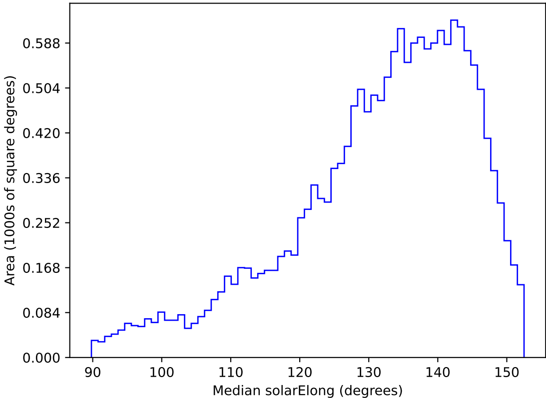
too_elab_r32_d2_giz_v3.4_10yrs WFD g band: Median solarElong
