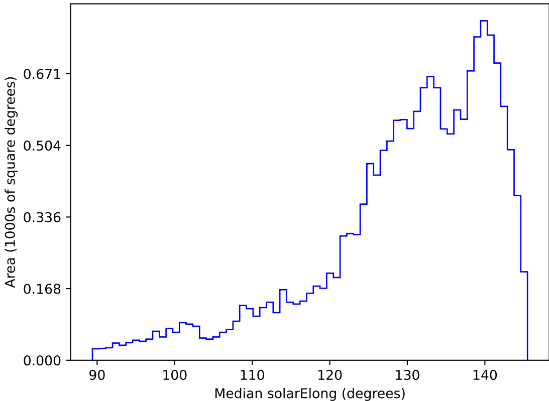
too_elab_r32_d2_giz_v3.4_10yrs WFD all bands: Median solarElong
