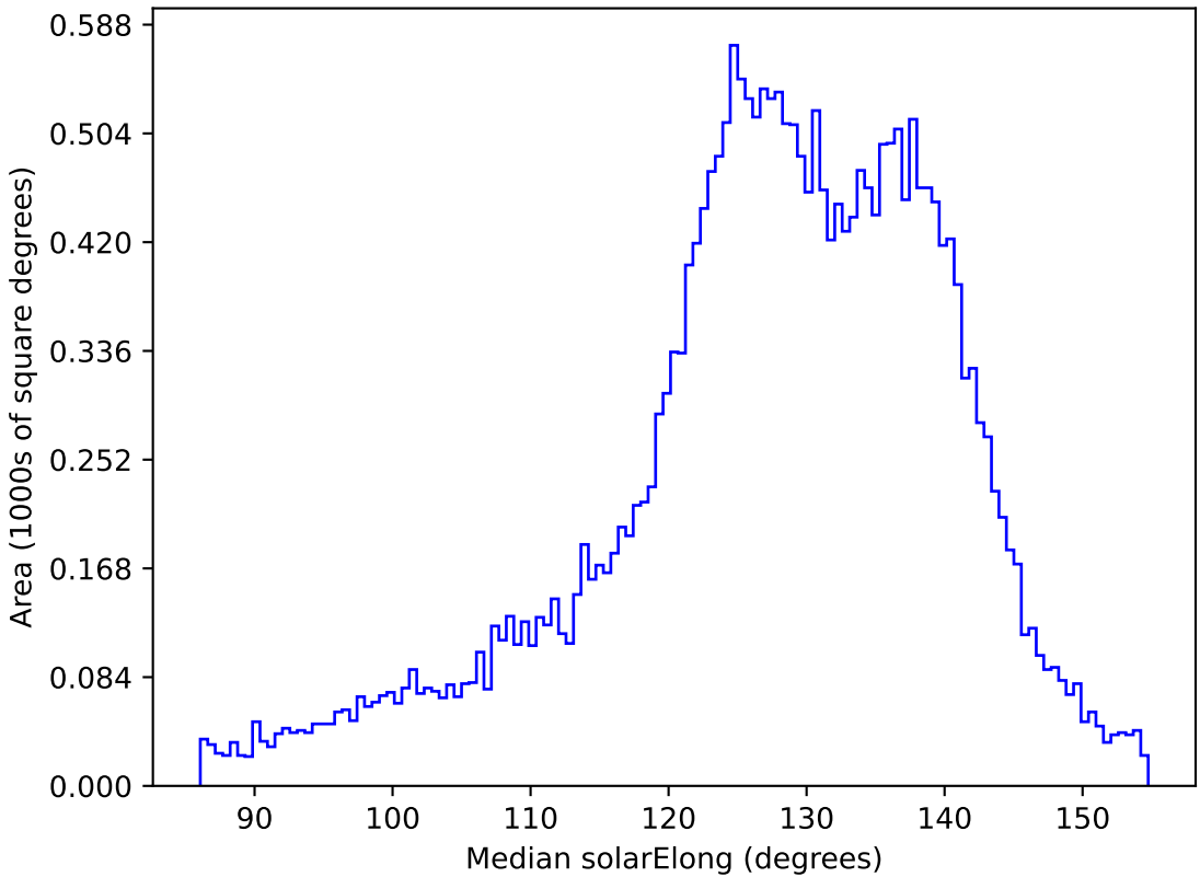
too_elab_r32_d2_giz_v3.4_10yrs All sky z band: Median solarElong
