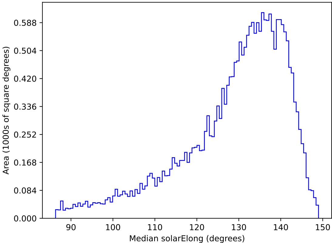
too_elab_r32_d2_giz_v3.4_10yrs All sky y band: Median solarElong
